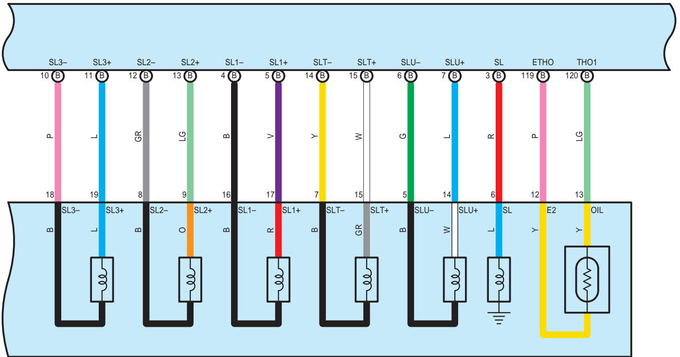
E8 ECT Solenoid (Transmission Wire)
