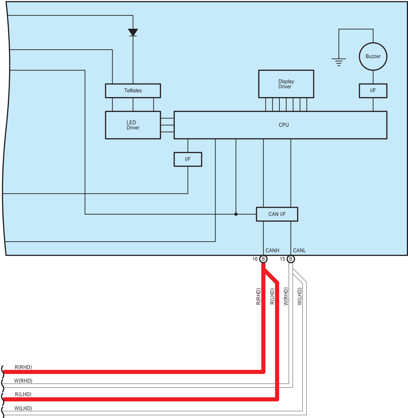
118(B) Combination Meter Assembly
