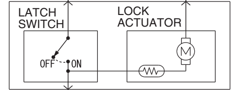
LATCH SWITCH and LOCK ACTUATOR
