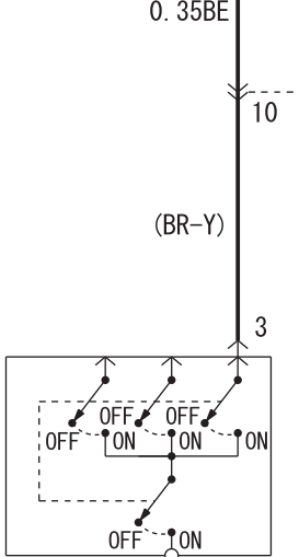
FRONT DOOR SWITCH (PASSENGER'S SIDE) (E-18)
