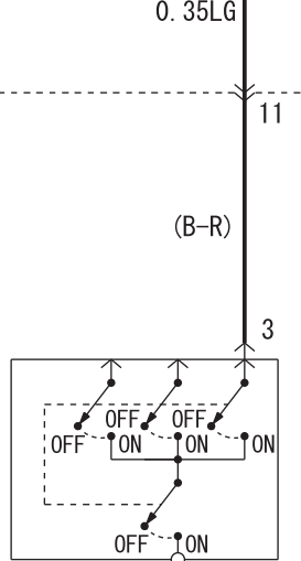
FRONT DOOR SWITCH (DRIVER'S SIDE) (E-04)
